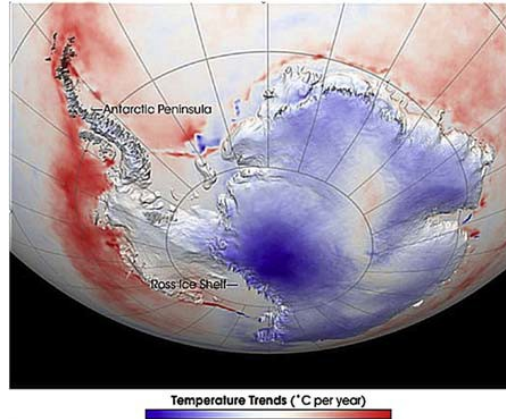
Figure 1. Antarctic temperatures (Blue = cooling, red = warming.) show that Antarctica is cooling, not warming
