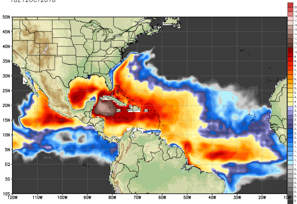
NCEP CDASv2 [CFSR Extension] TC Heat Potential [ \times 10^8 J/m 2 ] 18Z12OCT2018
