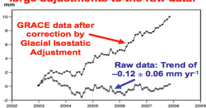
Fig. 1. Ocean mass change from GRACE over 2003–2008. The open circled curve is the raw time series. The black triangles curve corresponds to the GIA corrected time series.
