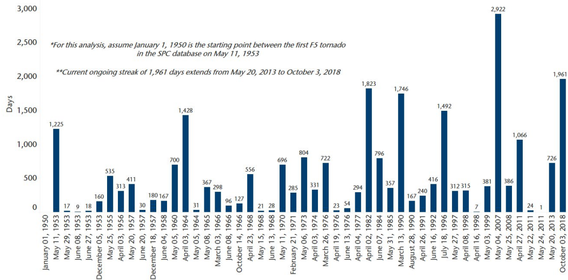
Days Between F5/EF5 U.S. Tornadoes (1950-2018)
