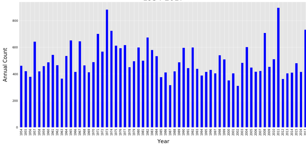
US Annual Count of (E)F-1+ Tornadoes 1954-2017
