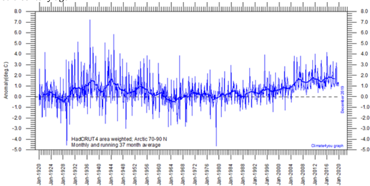
Figure 20: HadCRUT Area weighted Arctic 70-90N Monthly and 37 month average
