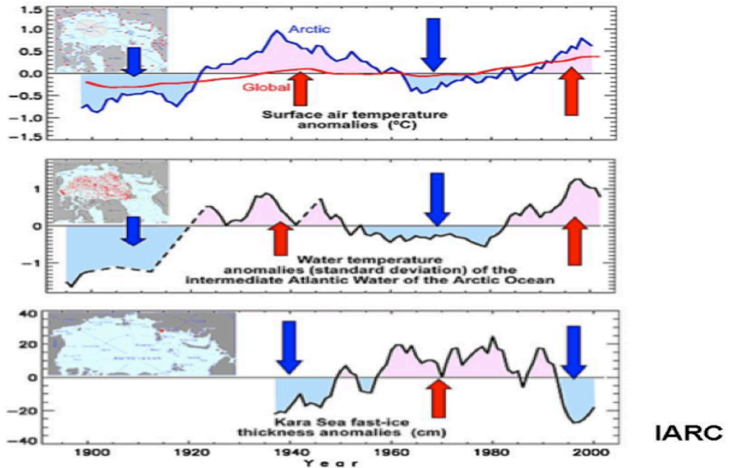
Figure 17: IAF IARC plot of arctic surface temperatures versus water temperatures in the intermediate Atlantic water of the Arctic ocean and Kara Sea fast-ice
