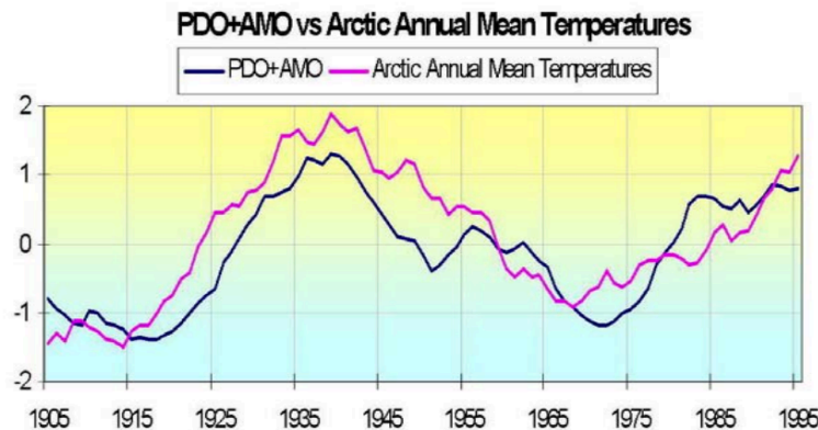
Figure 16: PDO+AMO versus Arctic Annual Mean Temperatures
