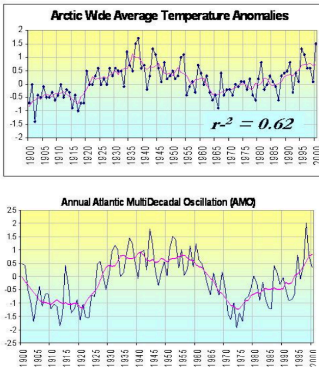
Figure 18: Arctic wide average temperature anomalies versus the annual AMO
