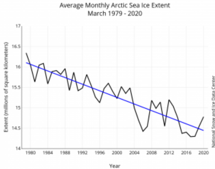
Figure 19: Monthly Arctic Sea Ice Extent (March 1979-2020)
