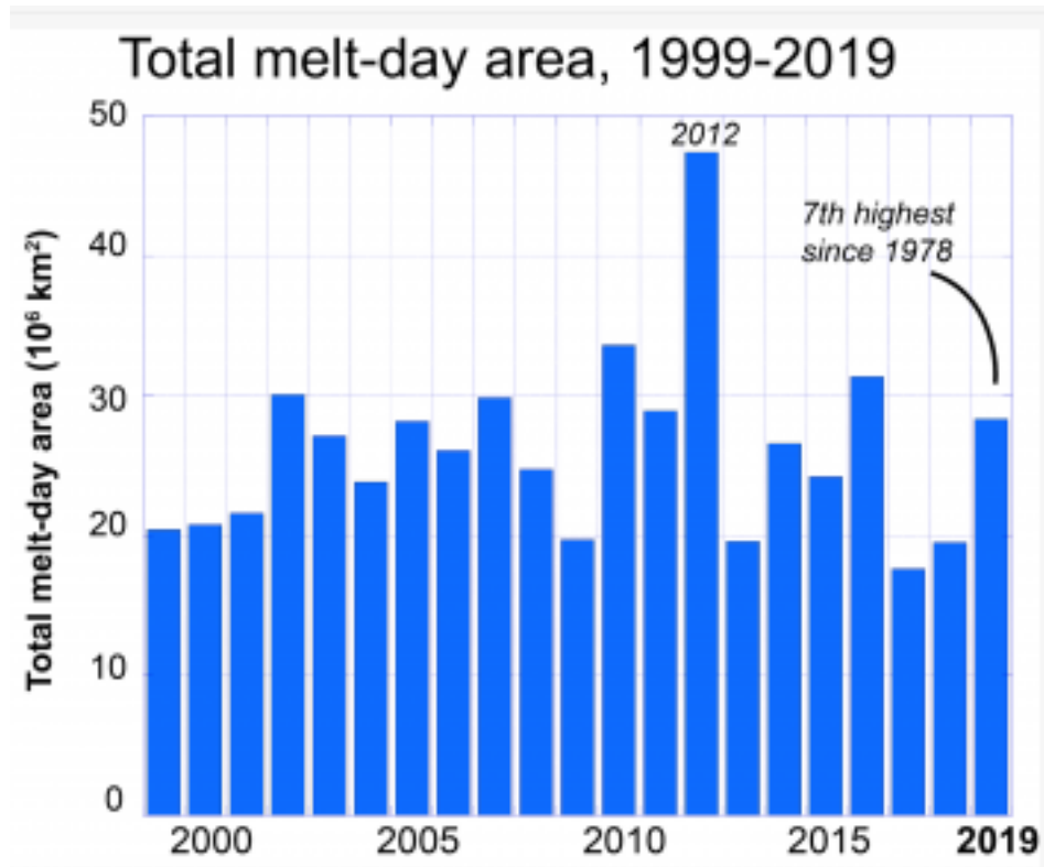
Figure 14: Greenland Melt-day Area since 1999
