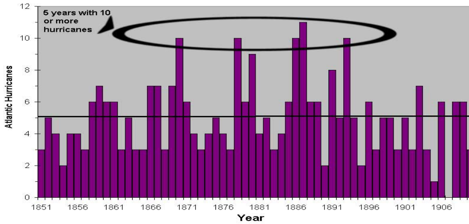
The average annual count for Atlantic hurricanes is 5.1.
