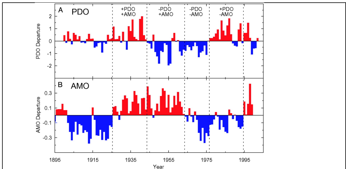
Time series of the annual PDO and AMO. Shaded areas indicate combinations of positive (+) and negative (-) PDO and AMO periods (McCabe etal)
